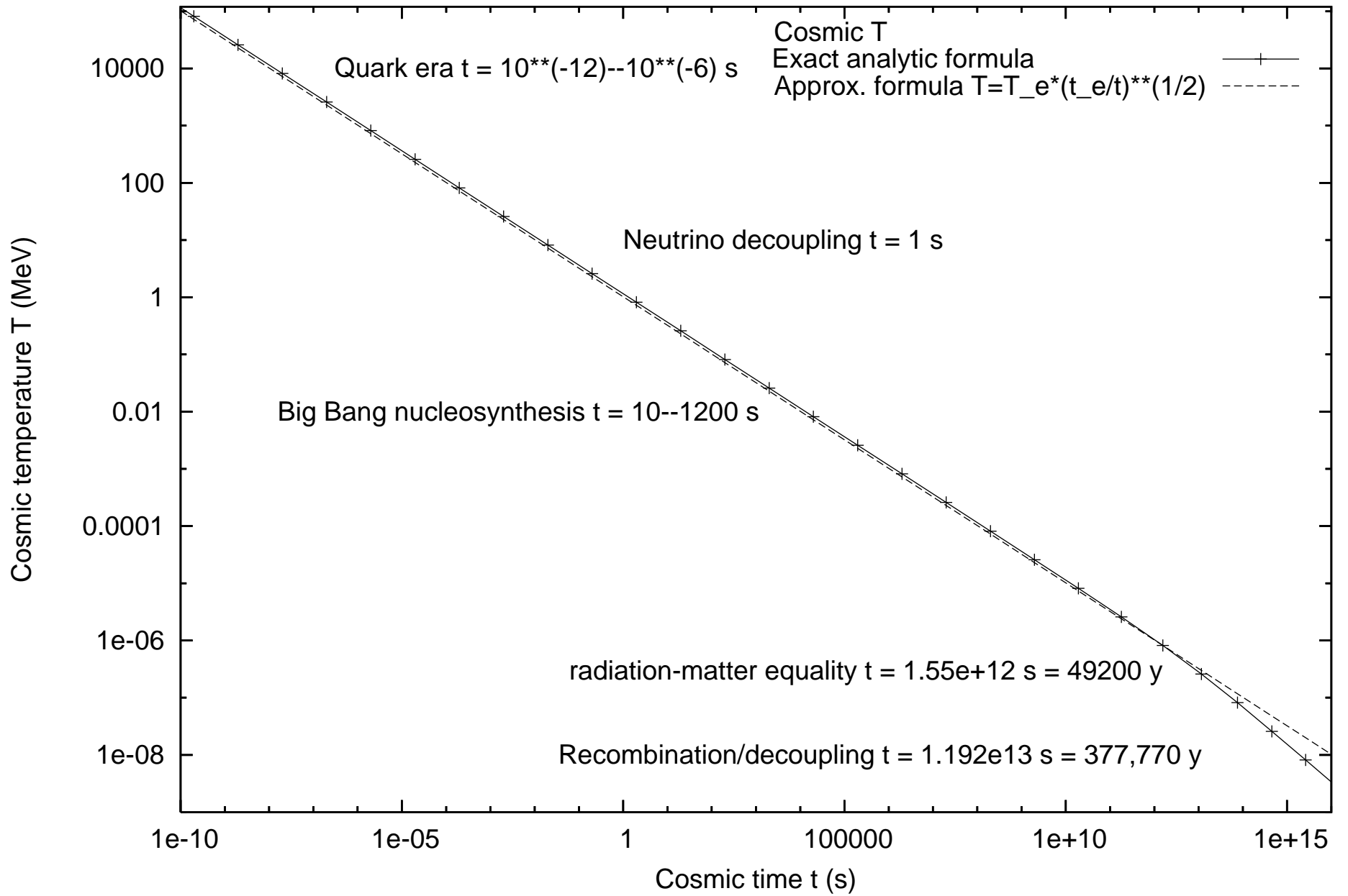
Cosmic temperature as a function of cosmic time
