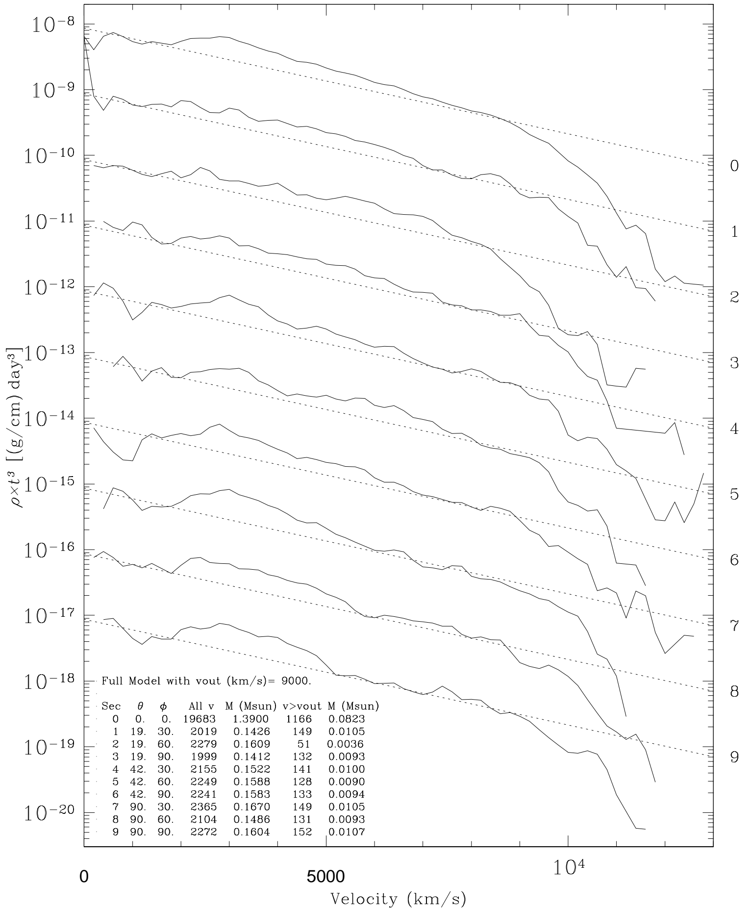
Densityplot in sectors for the Roepke model c3_3d_256_10s
