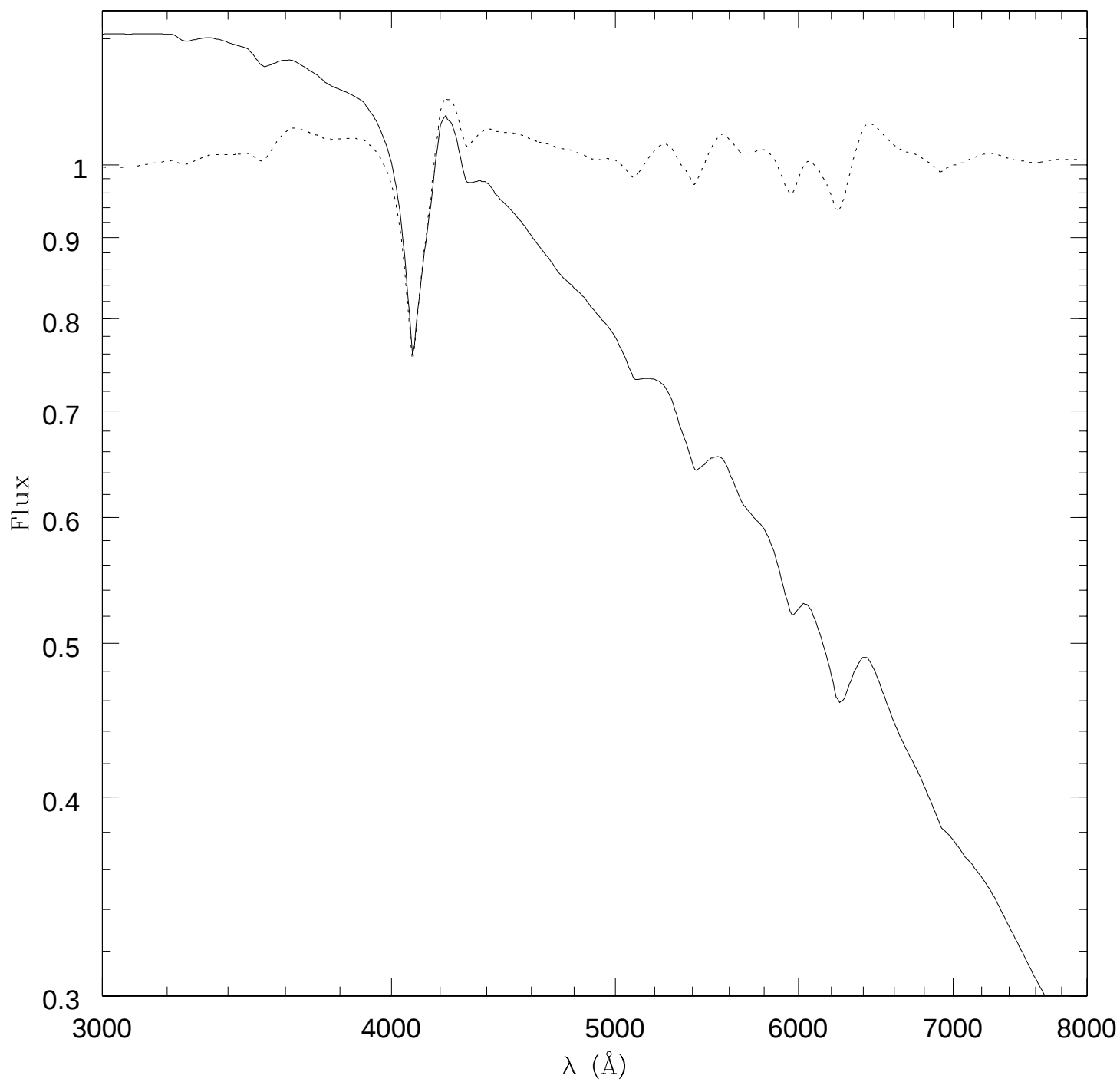
Ca I comparison
