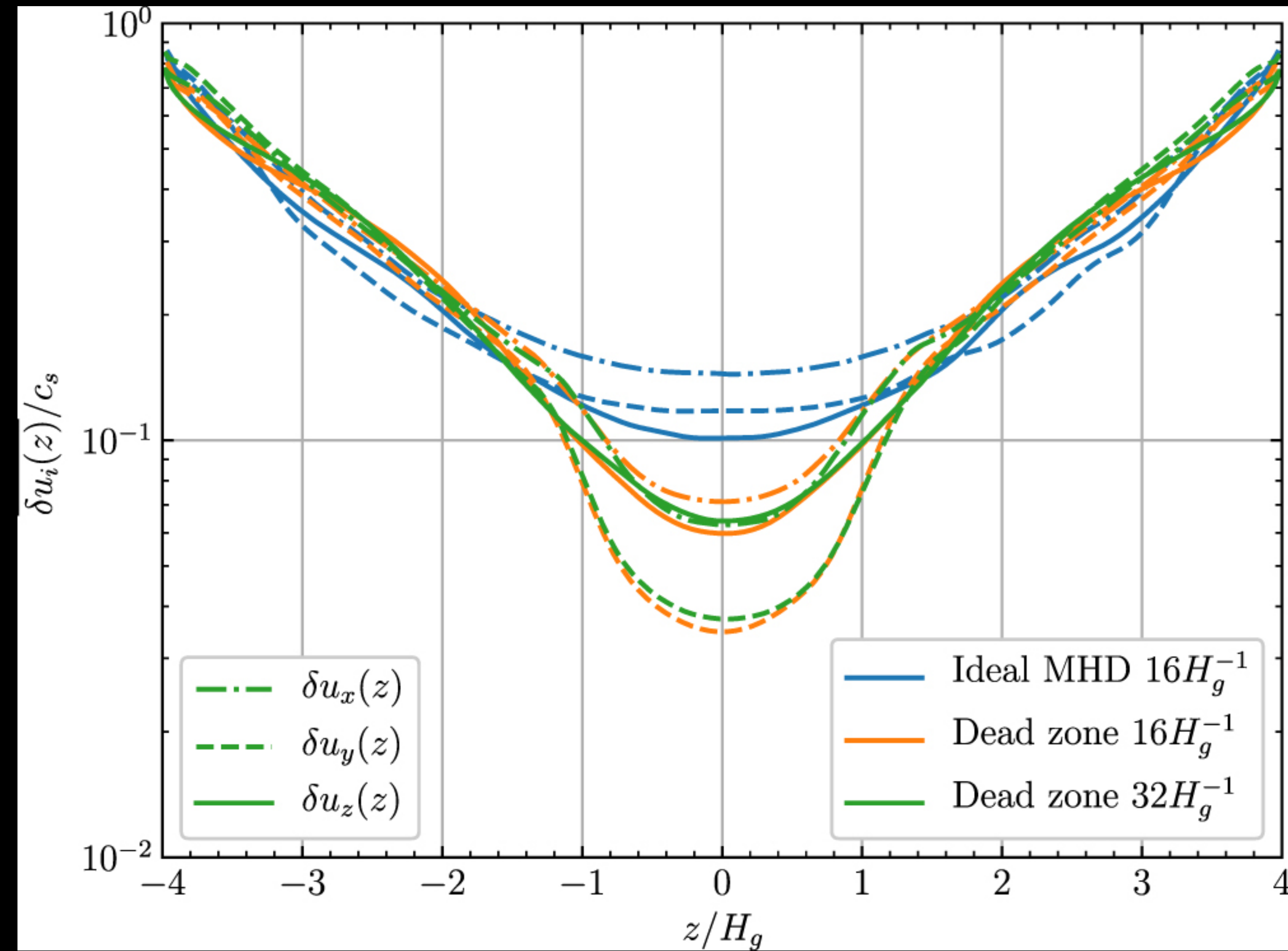
Yang, Mac Low, & Johansen (2018)
