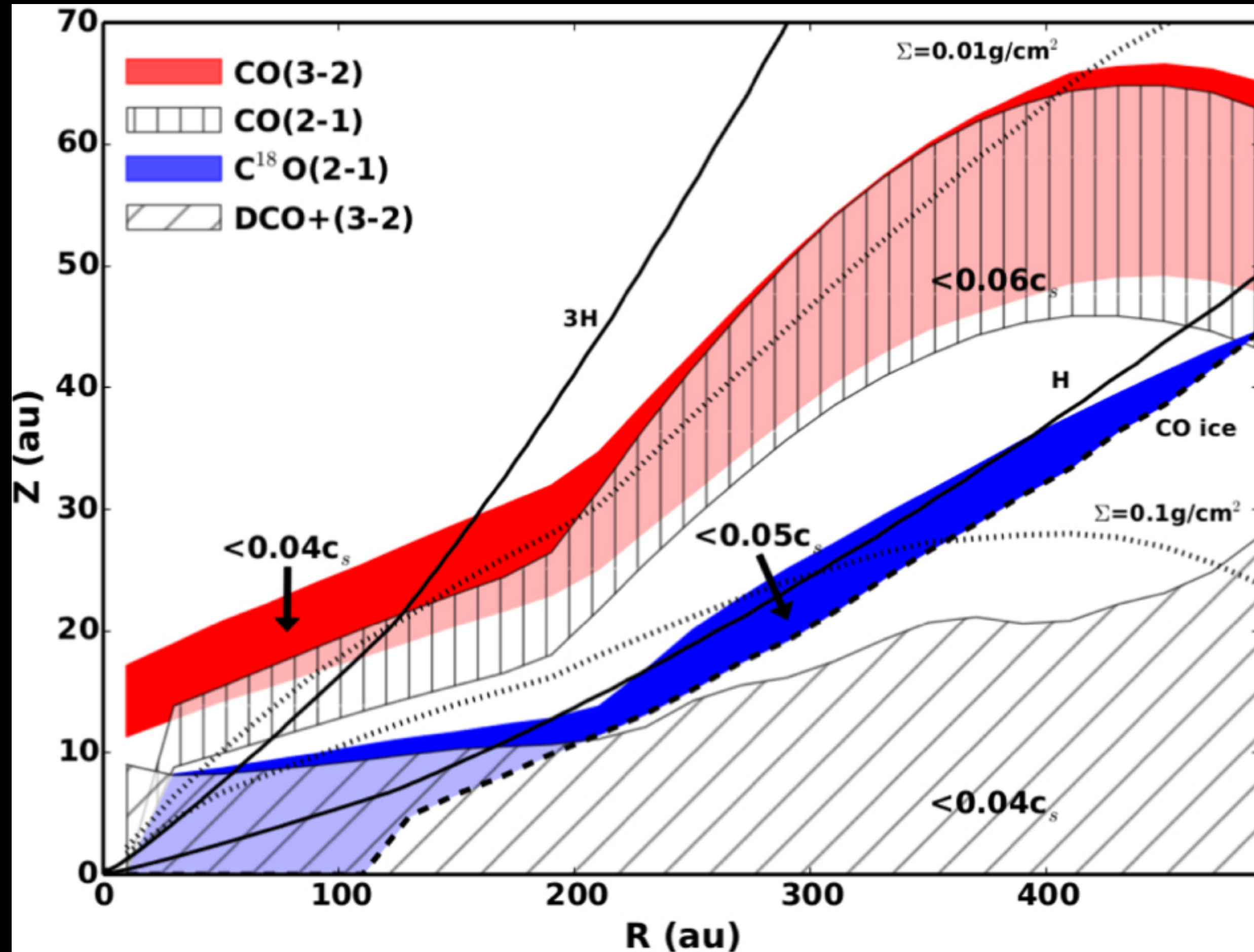
Flaherty et al. (2017)
