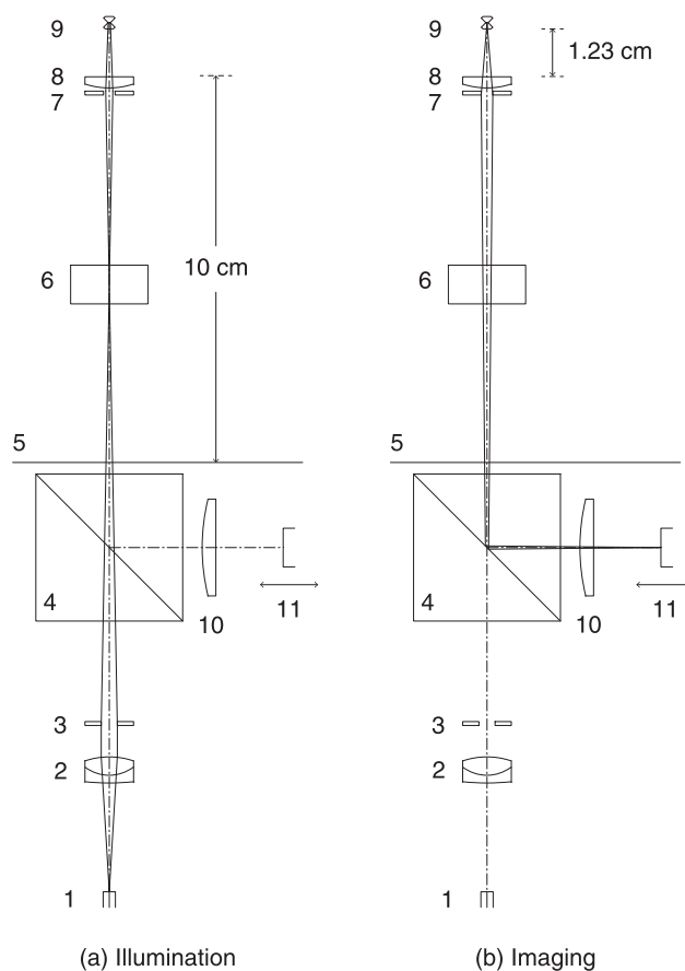
FIG. 3. Optical configuration for viewing the gasket and sample of a diamond anvil cell (DAC) placed inside the high pressure gas loading apparatus. (a) Light from optical fiber (1) is focused by lens (2) with aperture stop (3). The illumination beam assembly (1, 2, 3) is supported in an angle adjustable mount attached to the pellicle beam splitter cube (4), which is attached to the outside face of the pressure vessel (5). The light beam passes through a sapphire window (6), aperture (7), and ZnSe plano-convex lens (8), into the DAC (9). The image of fiber (1) by lens (2) is formed at or before window (6). (b) Light reflected from the DAC (9) is collected by the ZnSe lens (8) with its 3.0 mm aperture stop (7), passes through the sapphire window (6) out of the gas loading apparatus at (5), and is reflected by the pellicle (4). The reflected beam passes through plano-convex lens (10) to reach the imaging sensor surface (11) of the camera. Lens (10) is fixed on the beam splitter cube (4), and the image of the DAC (9) is brought into focus on the sensor surface (11) by moving just the camera.
