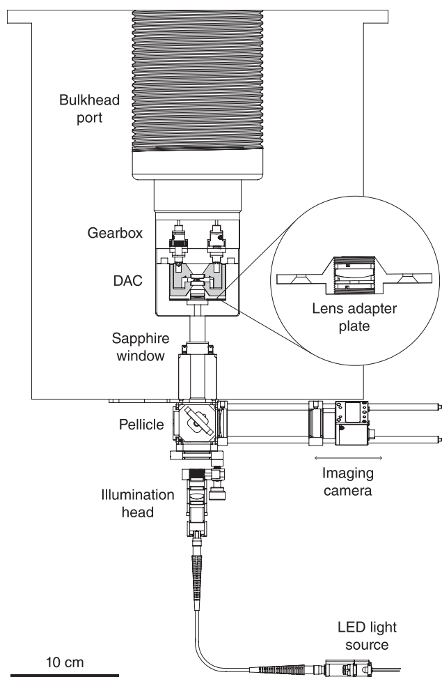
FIG. 1. A cross-sectional view of the high pressure vessel of the gas loading system, containing the gearbox with the diamond anvil cell (shaded) inside, and the imaging system attached to the underside.
