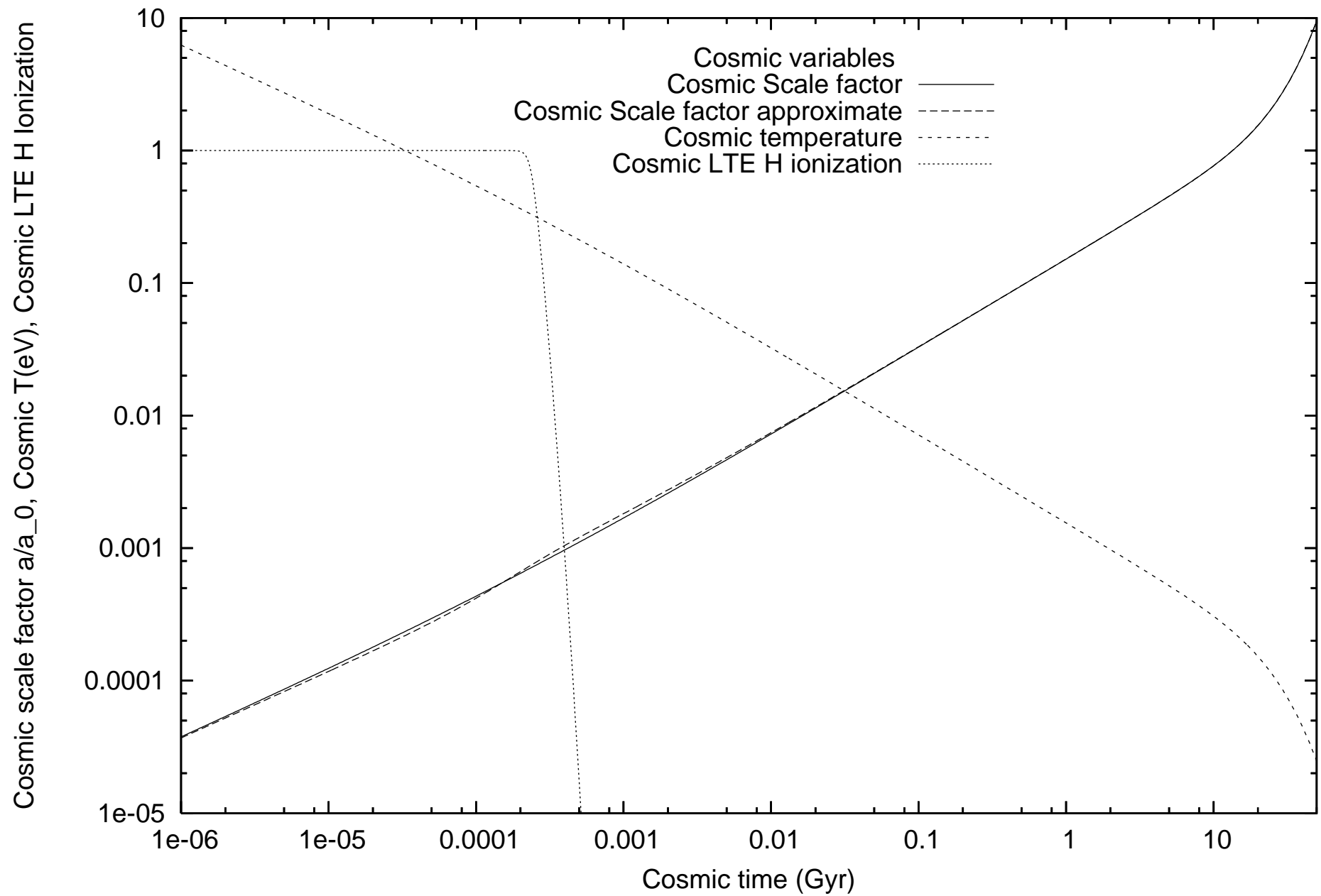
Cosmic Evolution for the Lambda-CDM model
